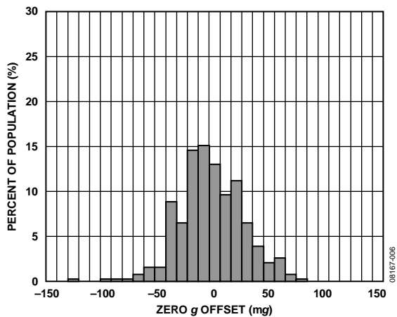
Figure 6. Z-Axis Zero g Offset at 25°C, V_s = 2.6 V
